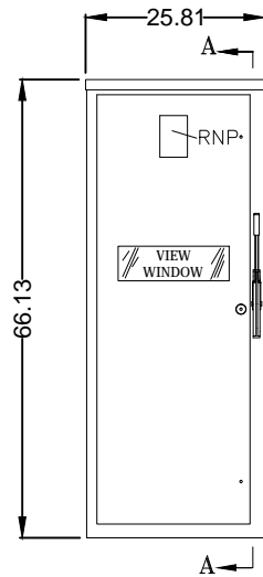
FRONT ELEVATION
