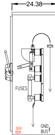
SECTION VIEW A-A
