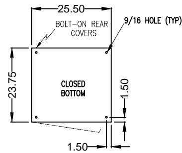
PLAN VIEW
